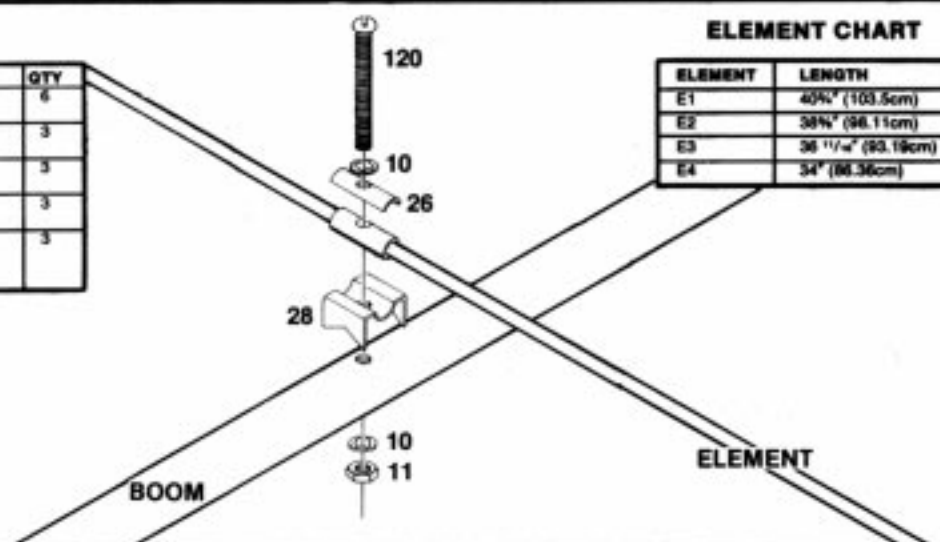
ELEMENT ASSEMBLY
