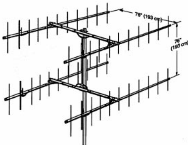
QUAD ARRAY (2) A147-22 & A147-SK HARNESS
