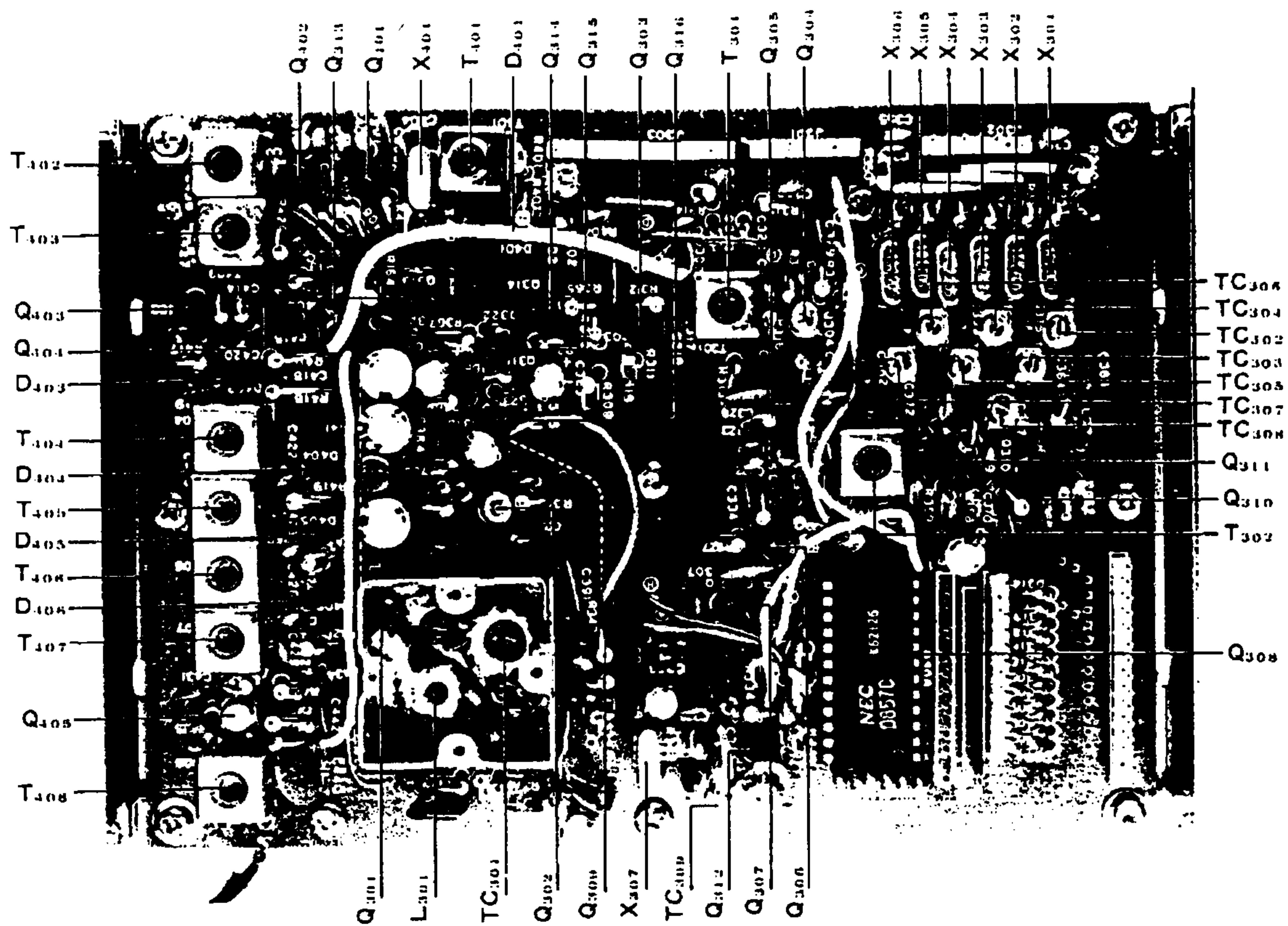
PLL UNIT
