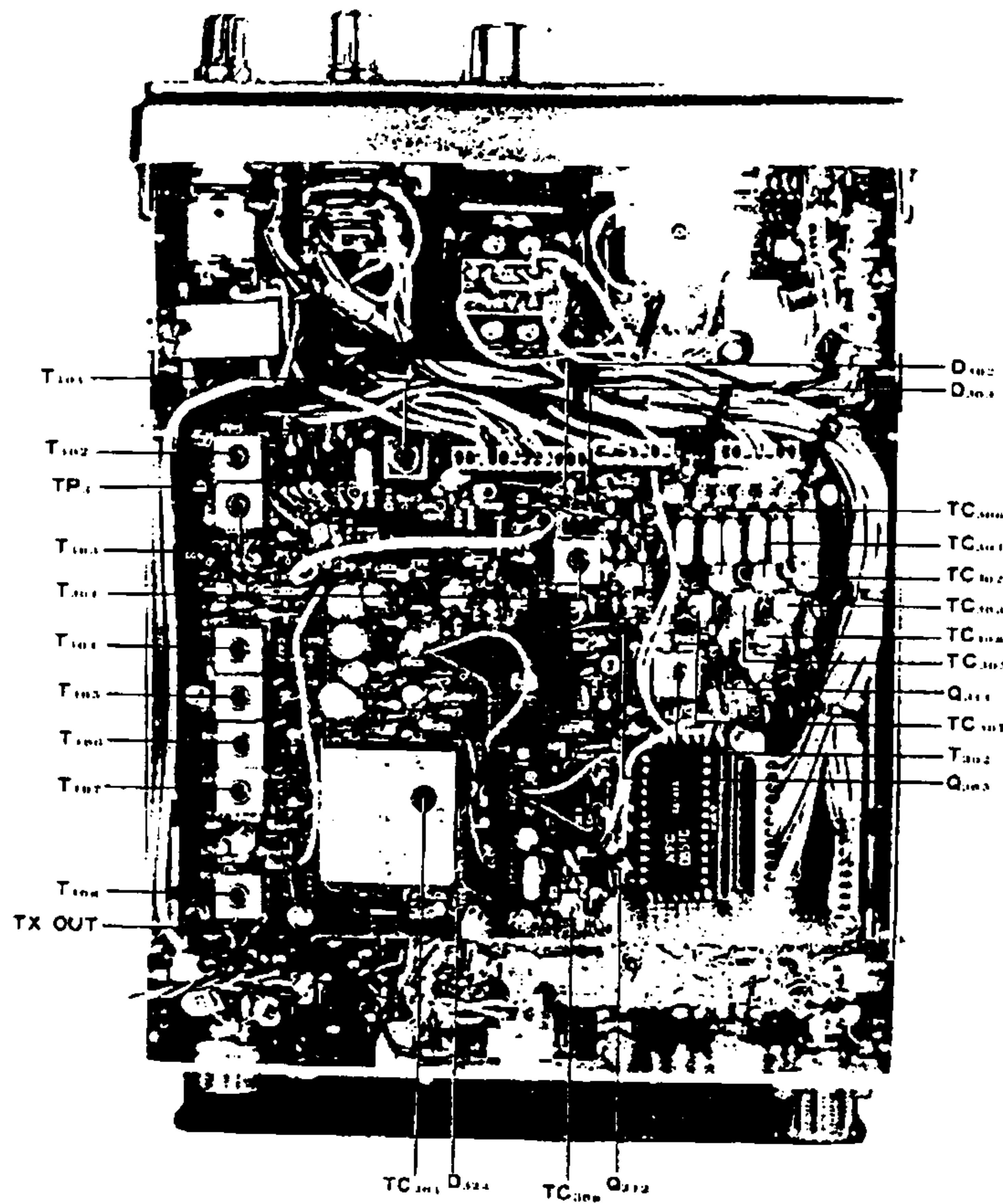
Figure 16 ALIGNMENT POINT
