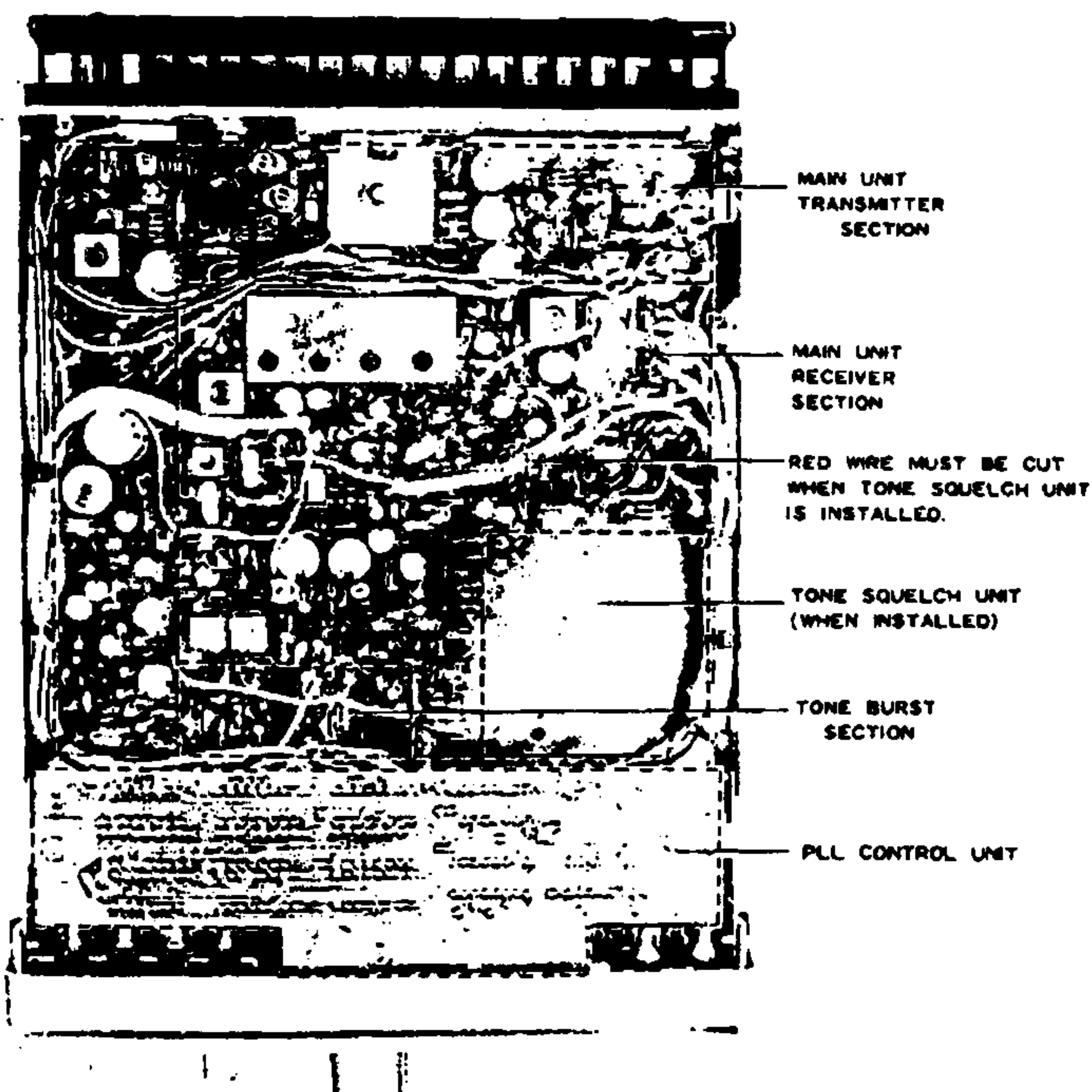
Figure 10 TOP VIEW
